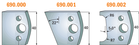
Profile knives cutting length=40mm (serie 690)
