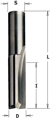
HW plunge centre tip
