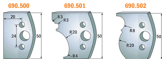
Profile knives cutting length=50mm (serie 690.5)
